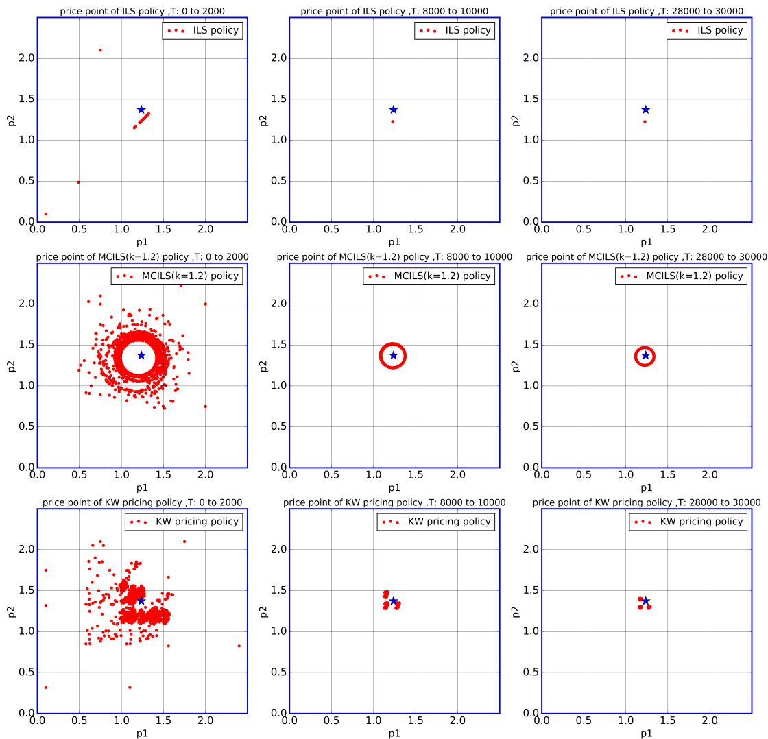
Figure 5: Illustration of the aggressive and slow optimizing strategies.
