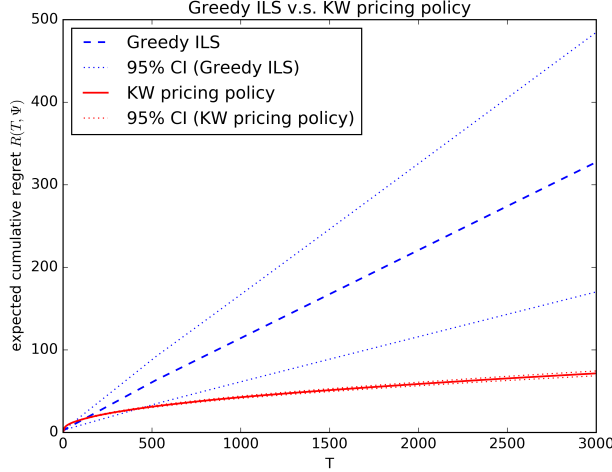
Figure 2: Comparisons between the ILS and KW pricing policies.
