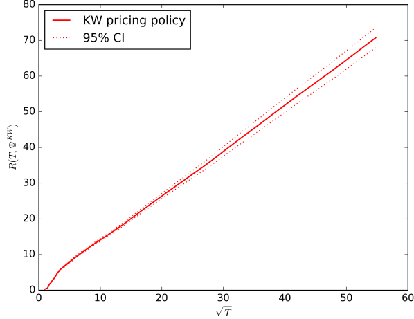
Figure 1: Average cumulative regret of the KW pricing policy.
