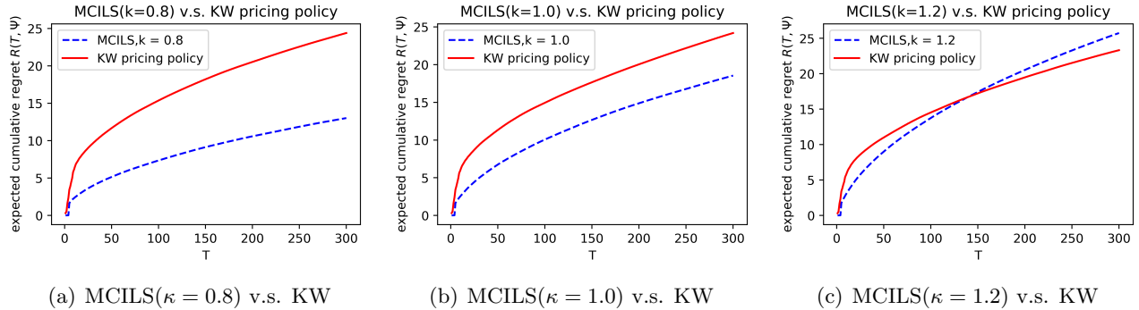
Figure 3: Comparisons between the MCILS( \kappa ) and KW pricing policies.
