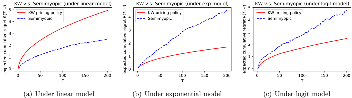
Figure 4: Comparisons between the semimyopic and KW pricing policies.
